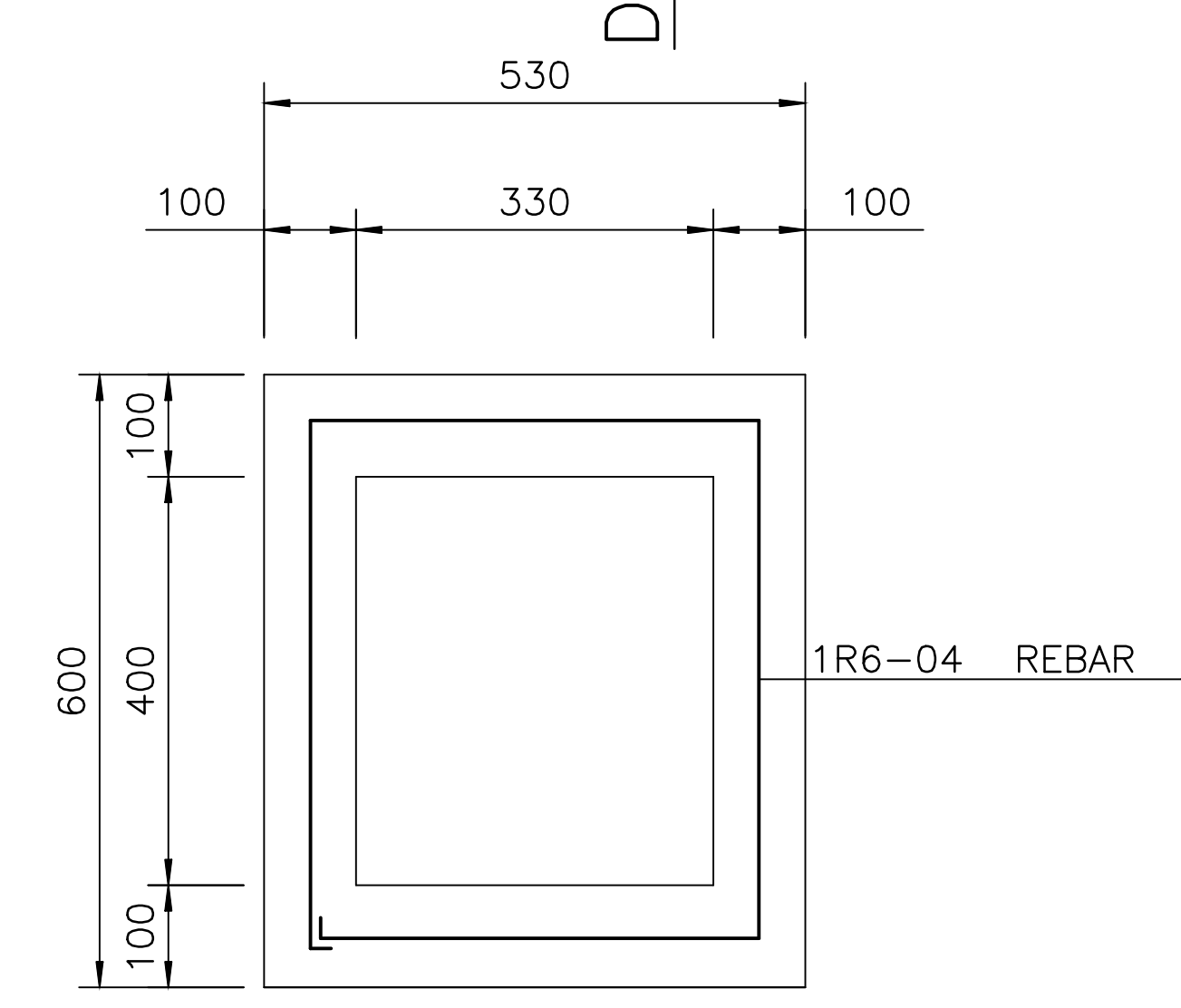
TYPICAL DETAIL OF MANHOLE SPACER RING 1 : 10
