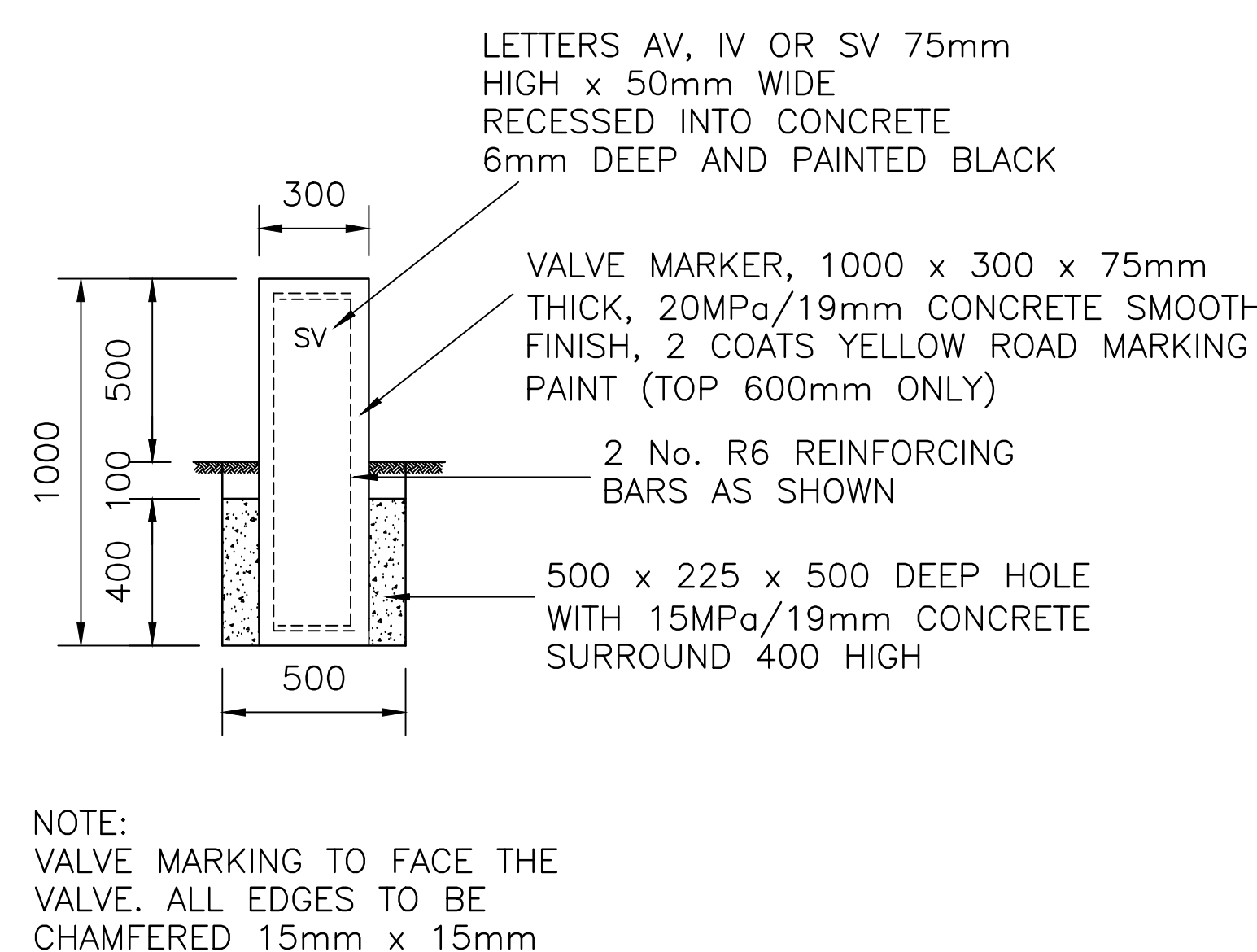
VALVE MARKER 1 : 25
