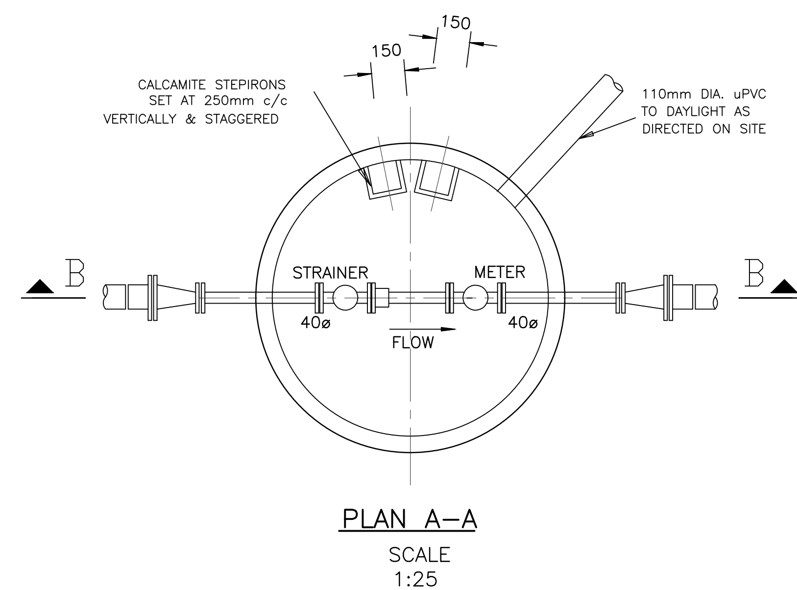
DETAILS OF CONTROL METER CHAMBER
