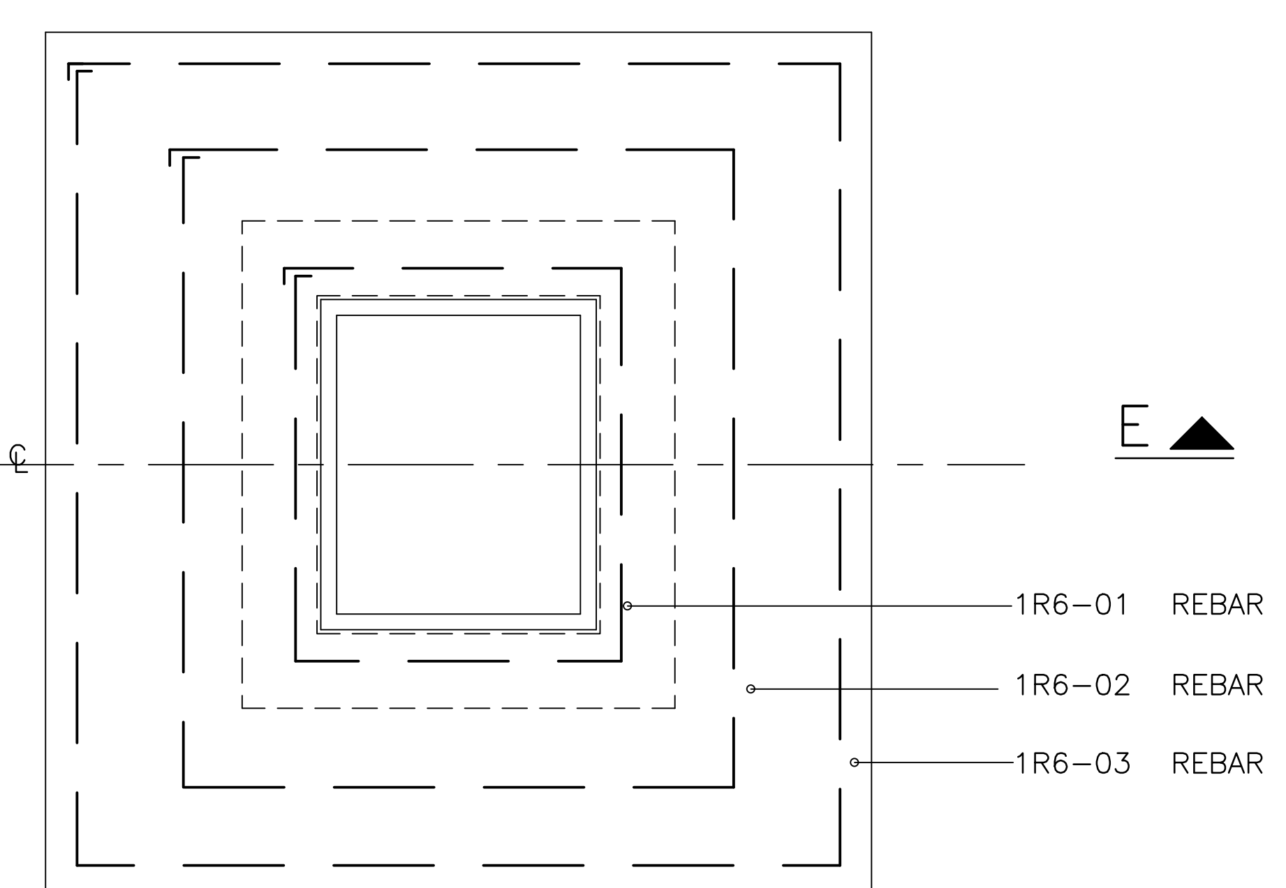
PLAN OF COVER REINFORCEMENT LAYOUT 1 : 10
