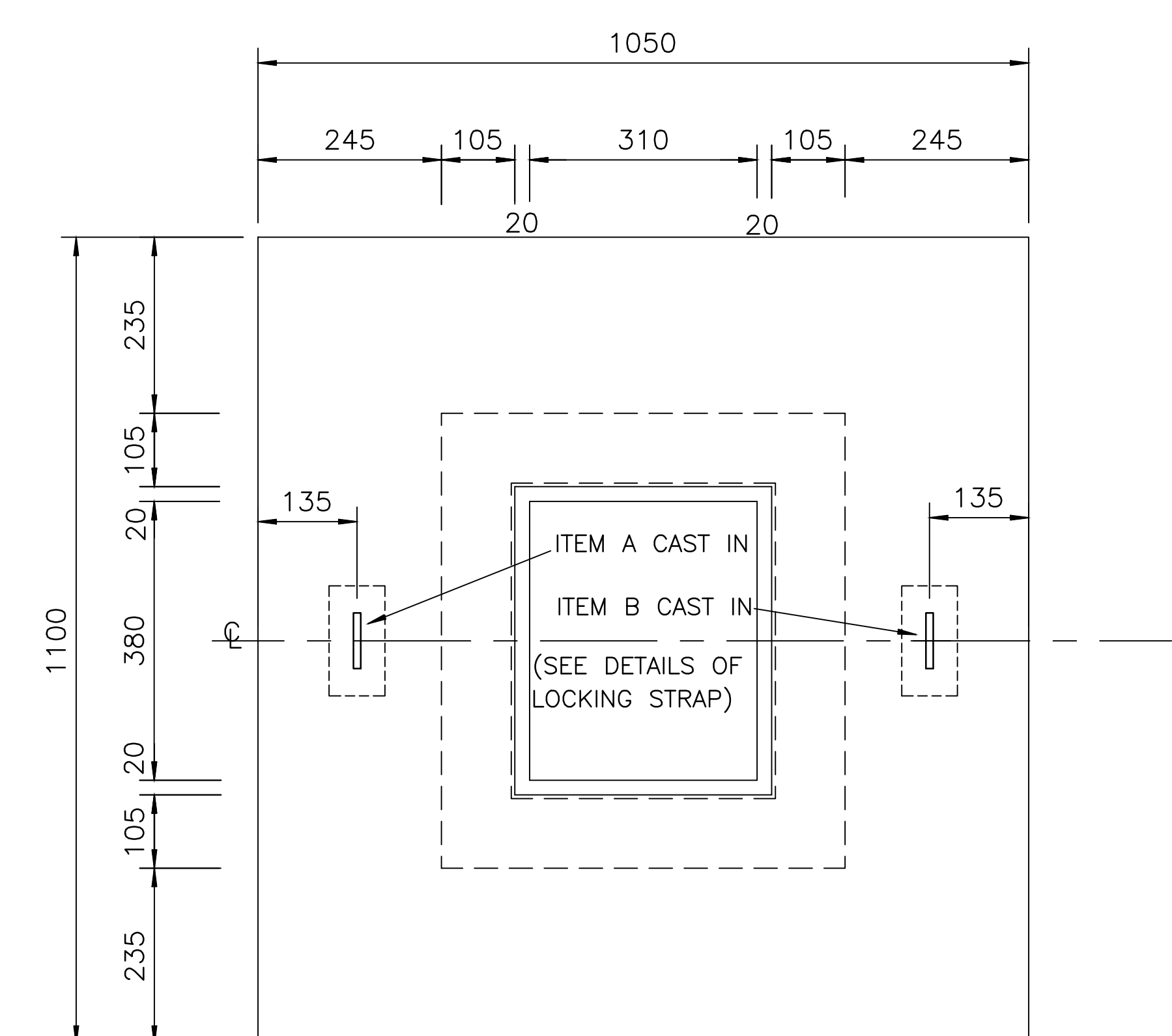
PLAN OF COVER CONCRETE LAYOUT 1 : 10
