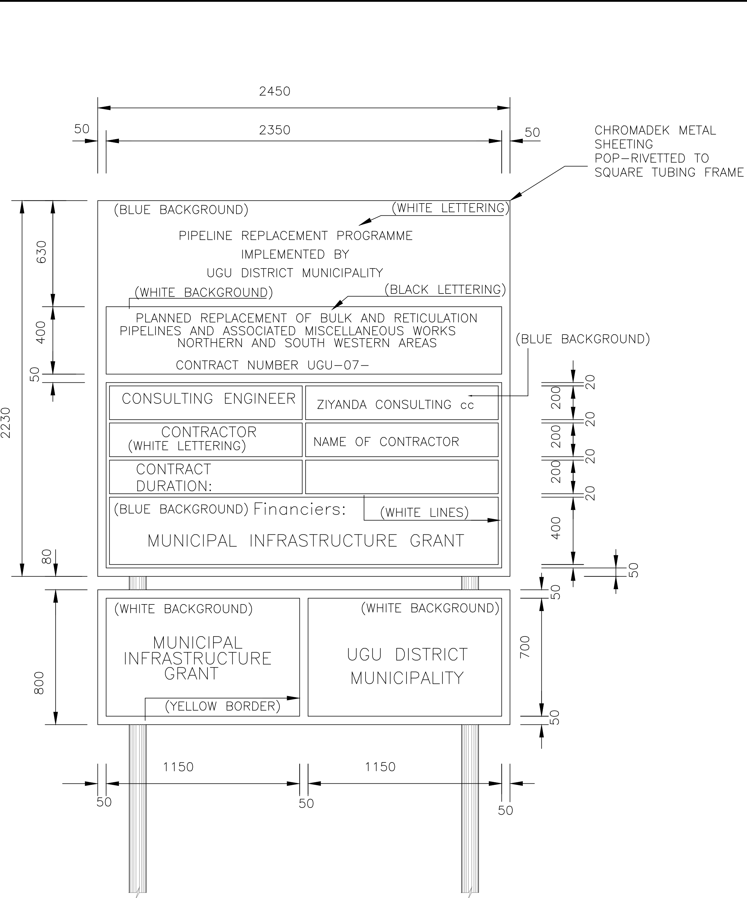
FRONT ELEVATION SCALE 1 : 20
