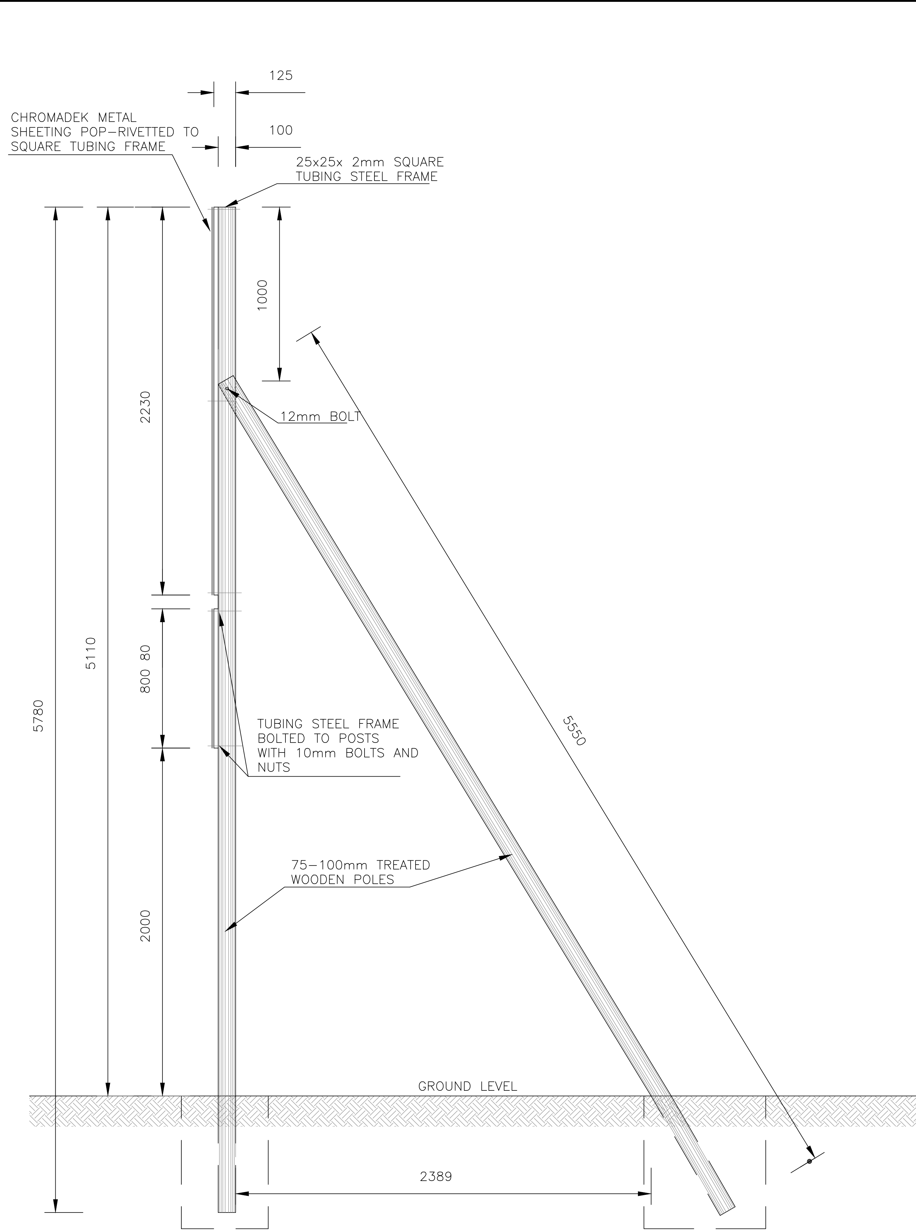
SIDE ELEVATION SCALE 1 : 20
