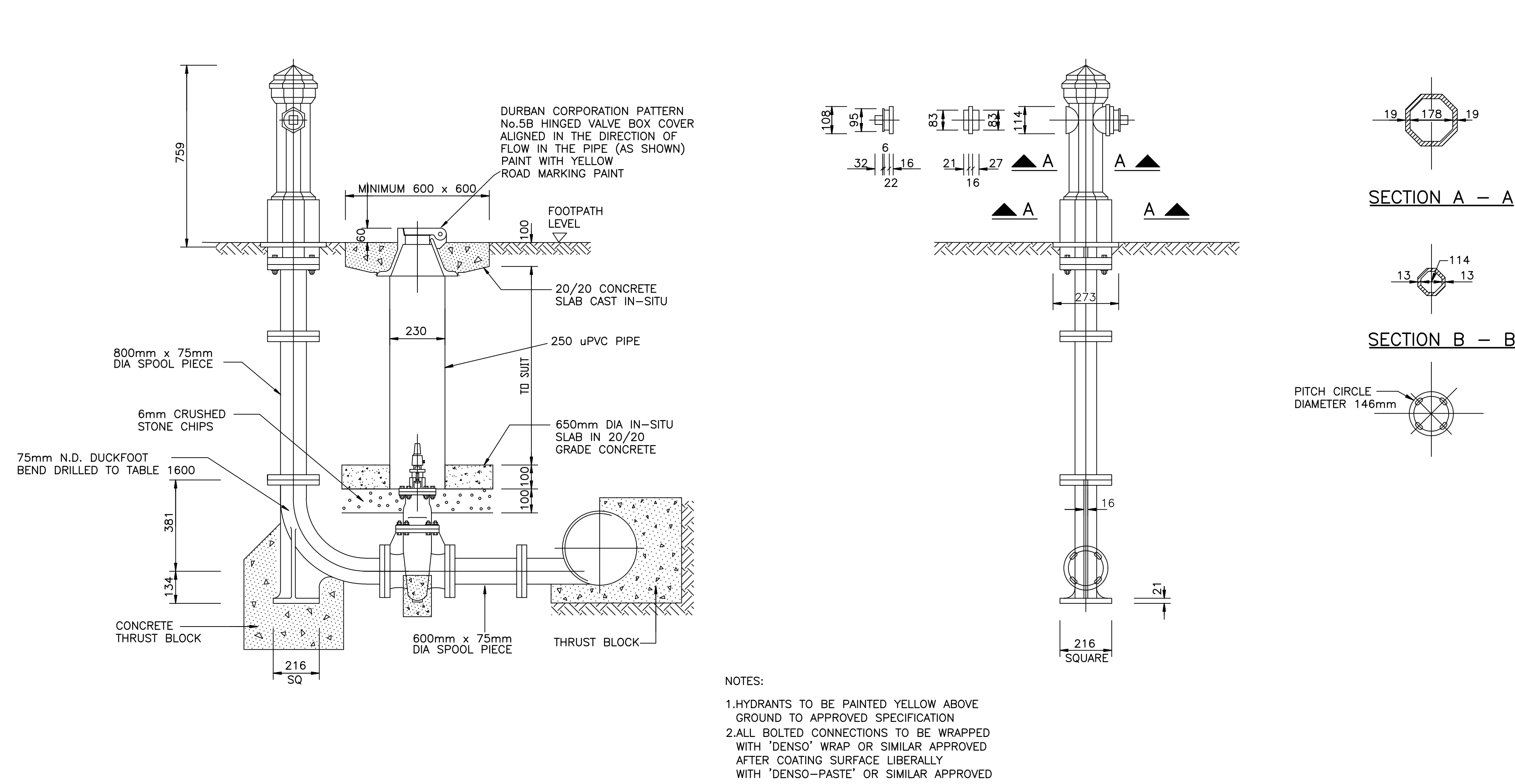
STANDARD 75mm DURBAN PATTERN HYDRANT N.T.S.
