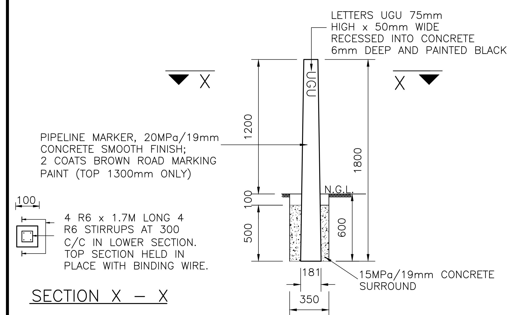
PIPELINE MARKER 1 : 25
