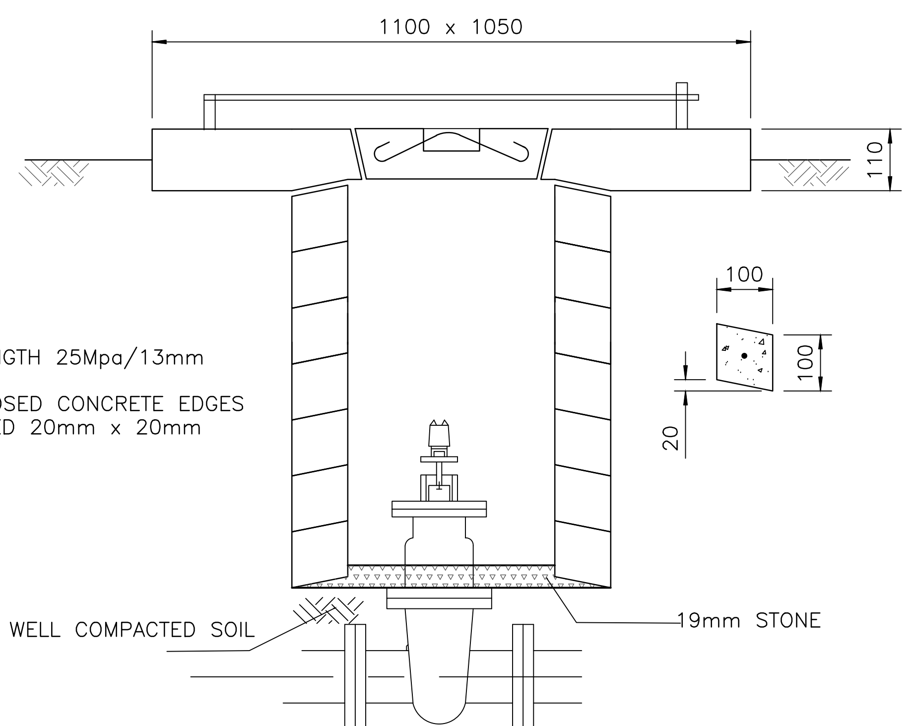
TYPICAL DETAIL OF MANHOLE USING SPACER RINGS 1:10
