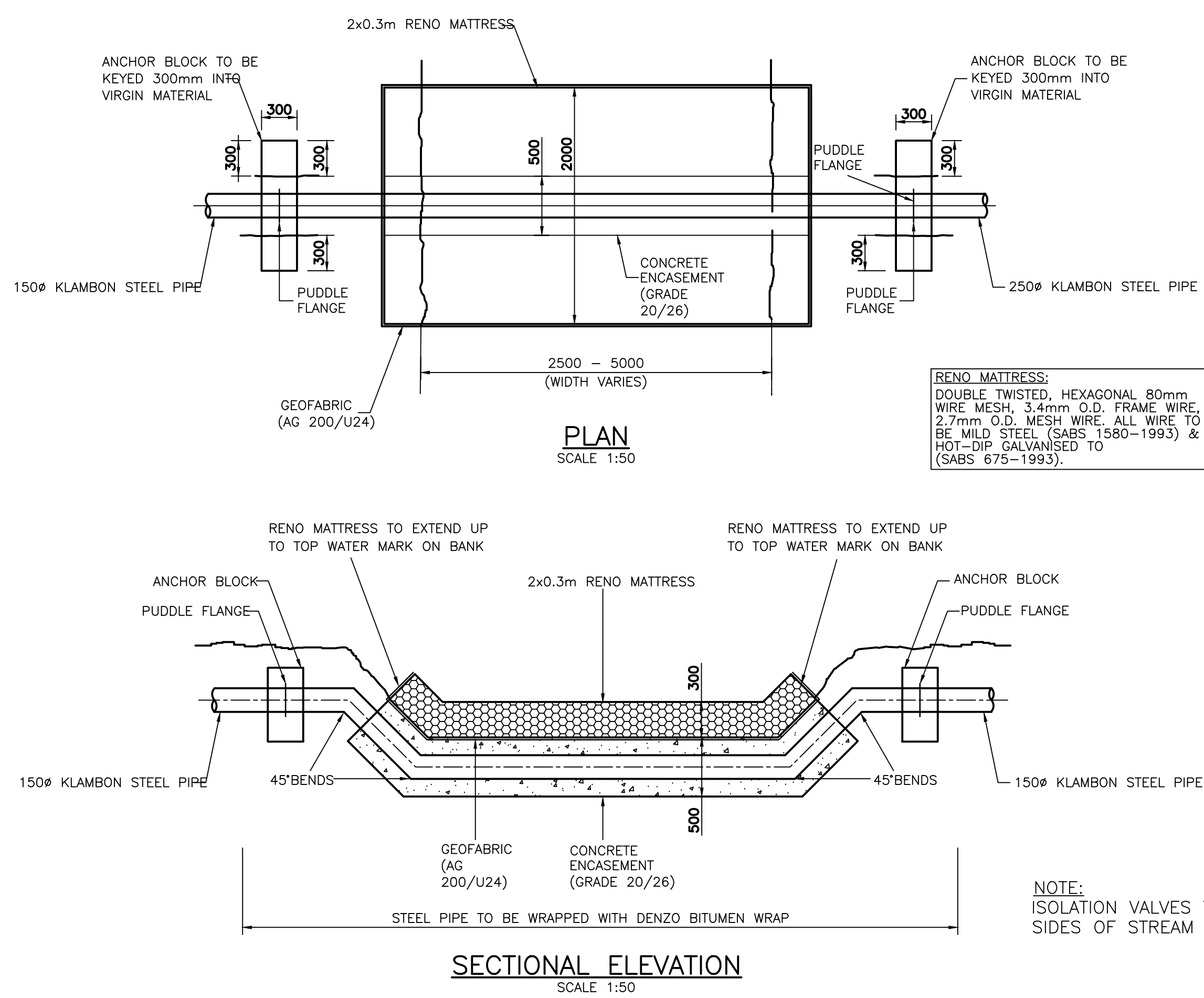
PIPELINE STREAM CROSSING DETAILS FOR STEEL/mPVC/HDPE PIPELINE
