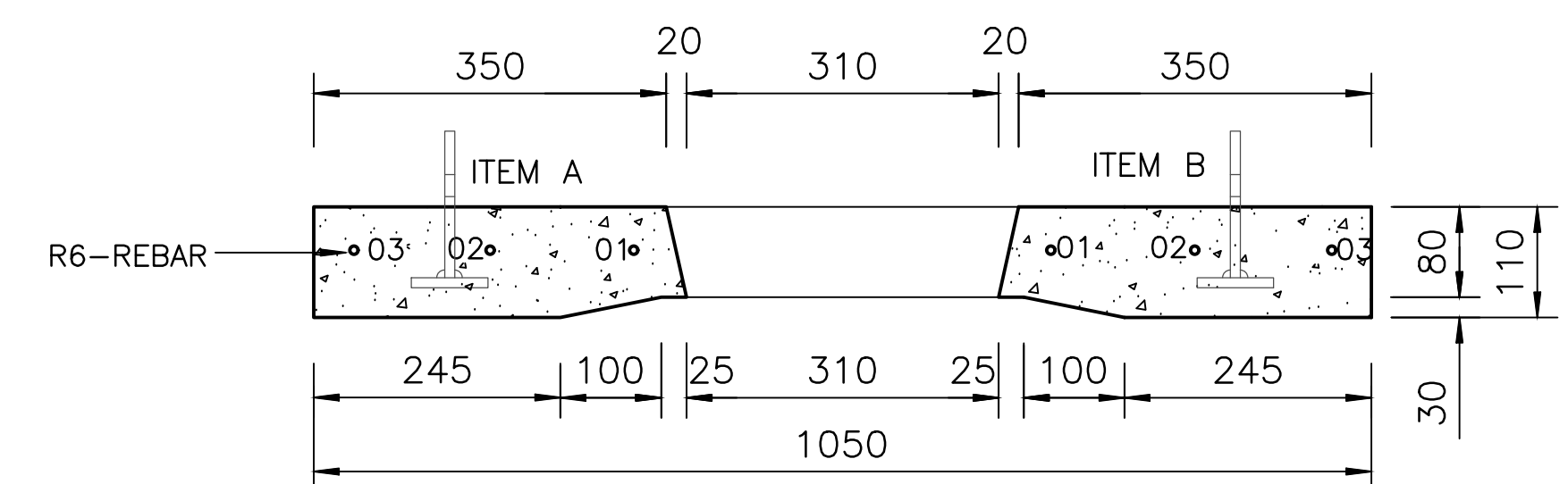
COVER SECTION E-E 1 : 10
