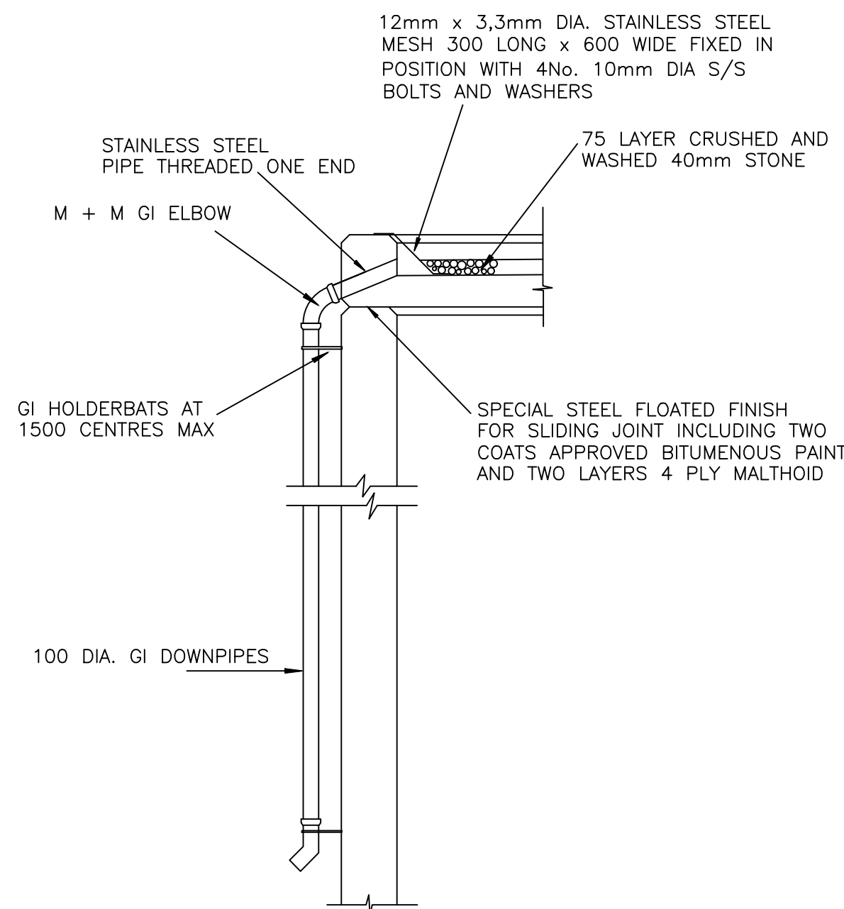
DETAIL OF ROOF RAIN WATER OUTLET
