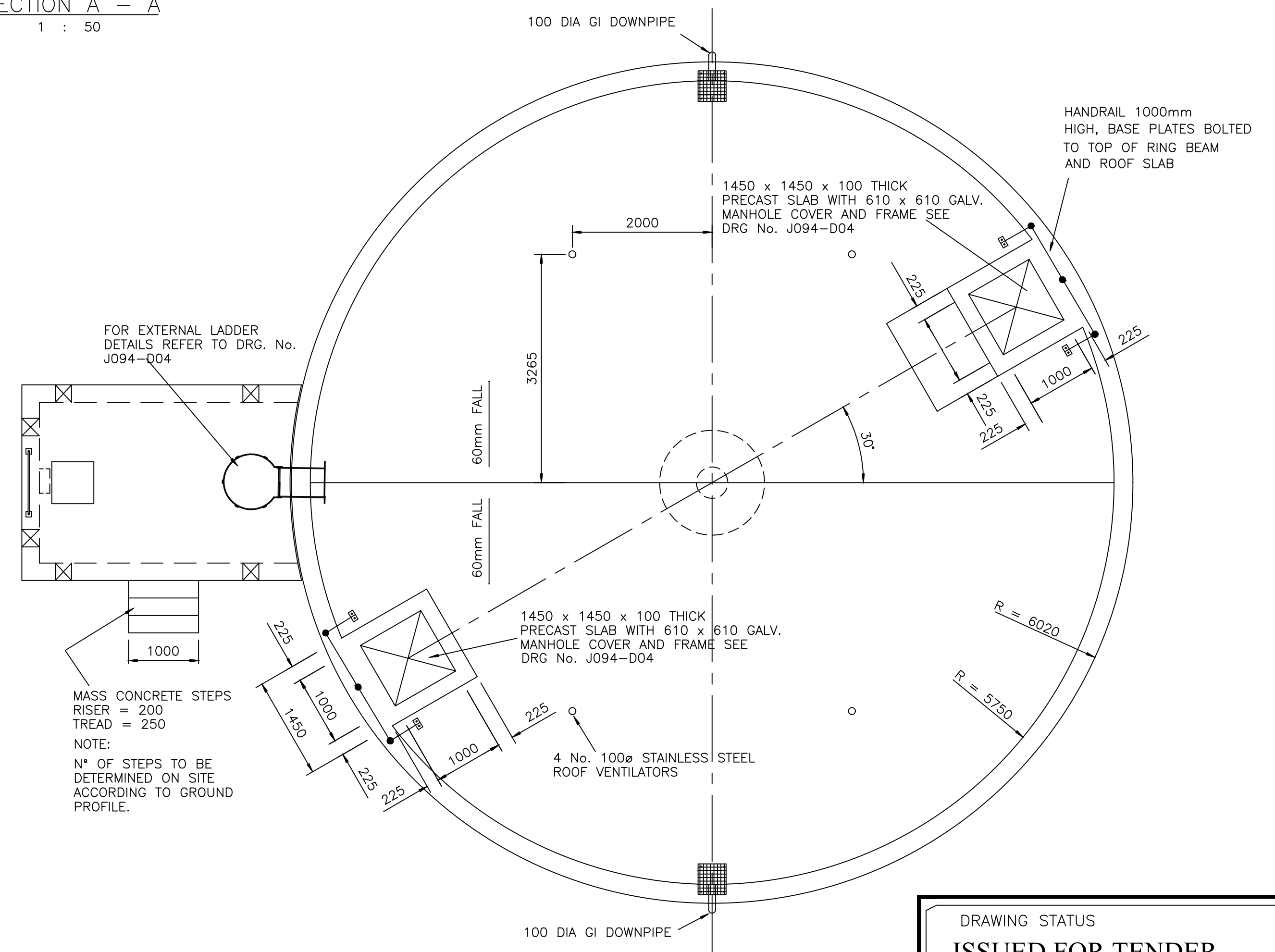
PLAN ON ROOF
