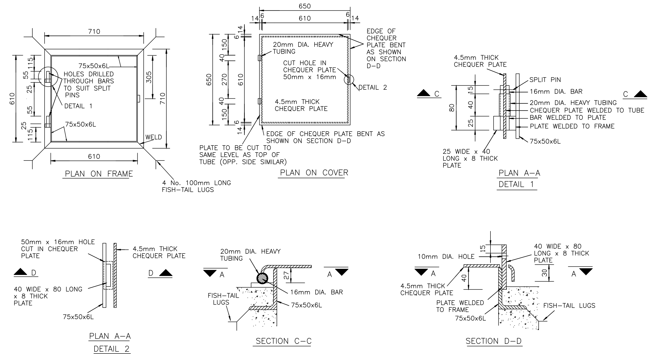
DETAILS OF GALVANISED MANHOLE COVER AND FRAME
