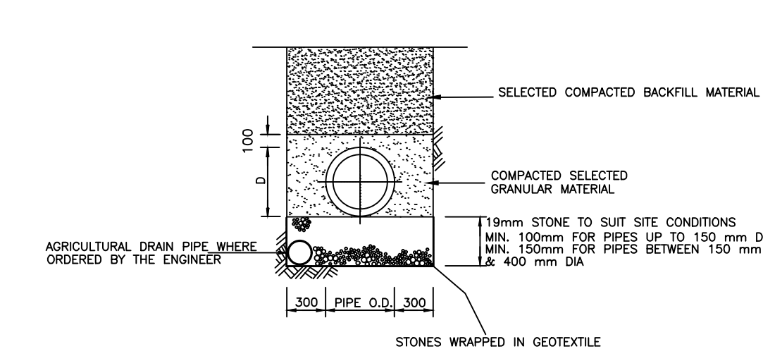
TYPICAL PIPELINE TRENCH SECTION N.T.S.
